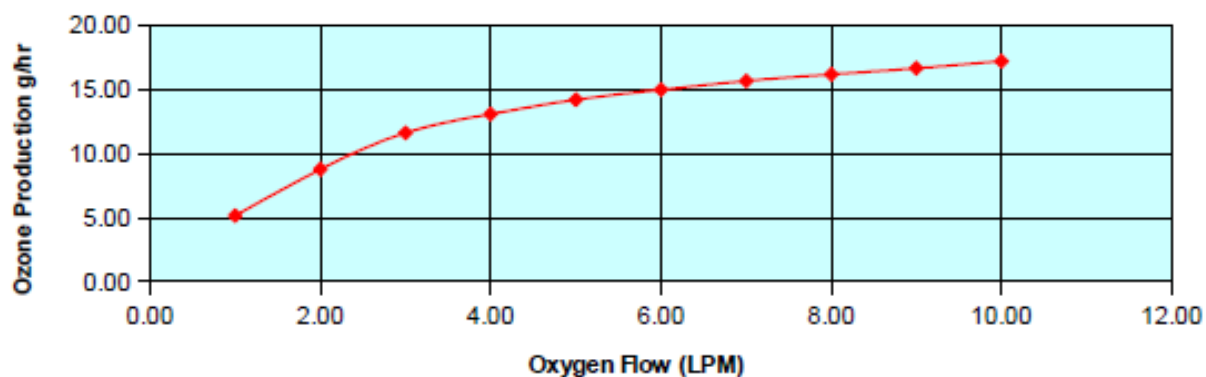
Ozone Production
