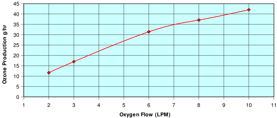
Ozone Production
