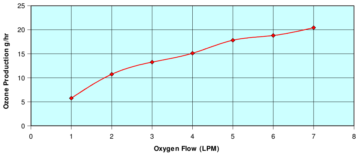
Ozone Production
