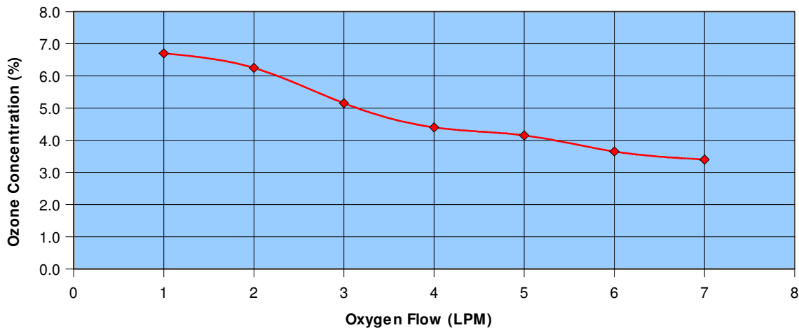
Ozone Production
