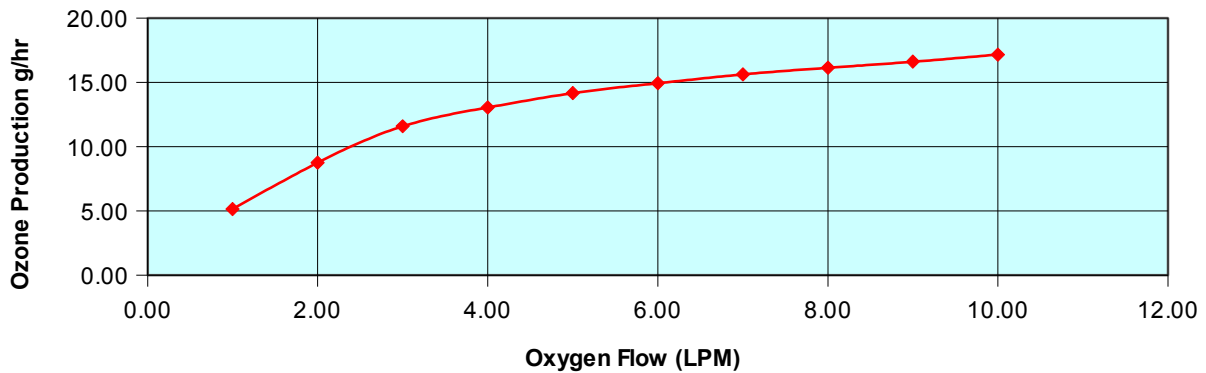
Ozone Production
