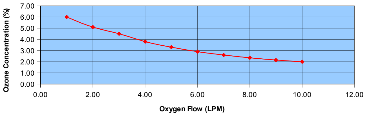
Ozone Concentration
