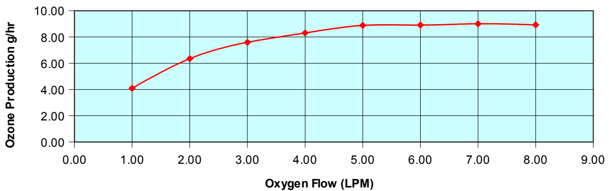
Ozone Production
