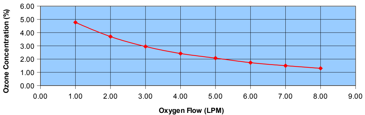
Ozone Concentration
