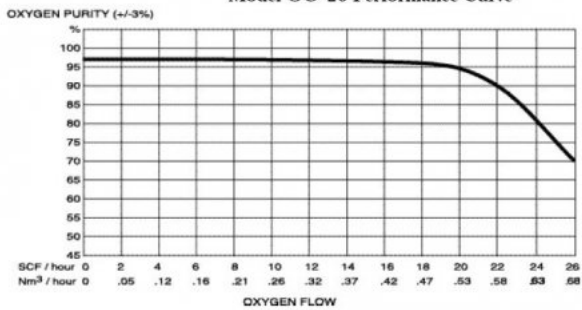
Model OG-20 Performance Curve
