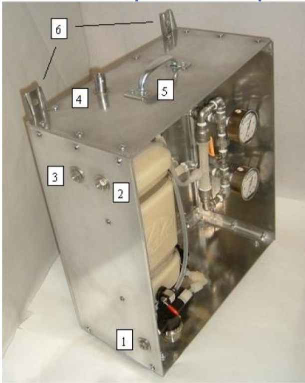
(1) 1/4" FPT water inlet, (2) 1/8" FPT ozone inlet, (3) 1/4" FPT water outlet, (4) 1/4" FPT ozone vent, (5) handle, (6) mounting brackets
