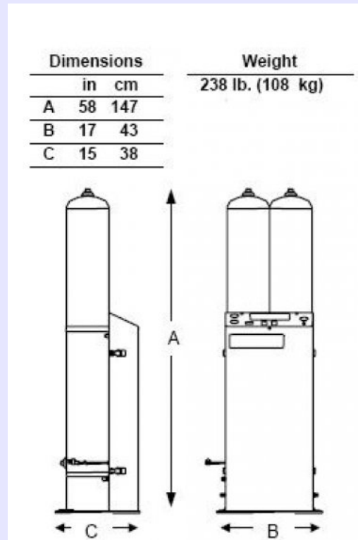
AS-B Dimension drawing
