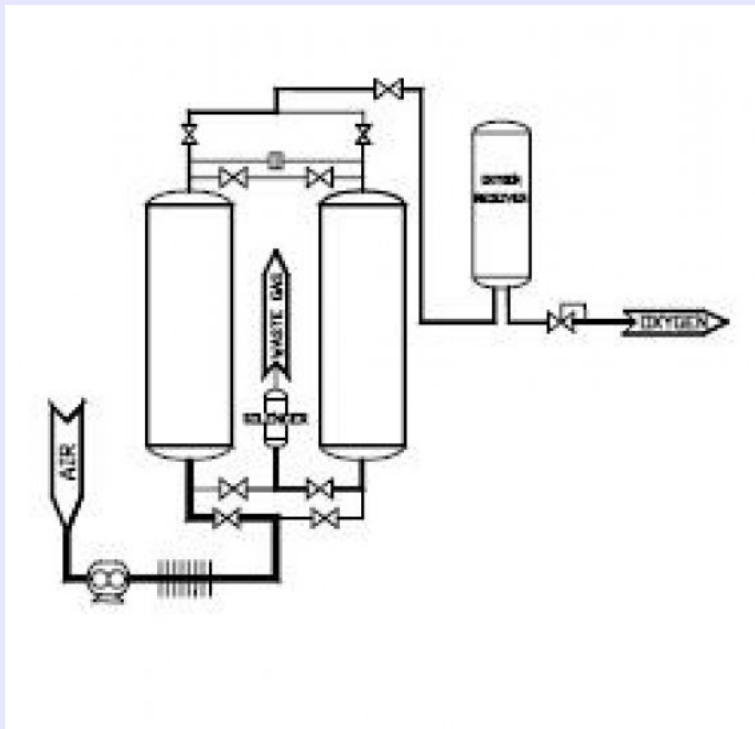
Diagram of the entire Oxygen System process
