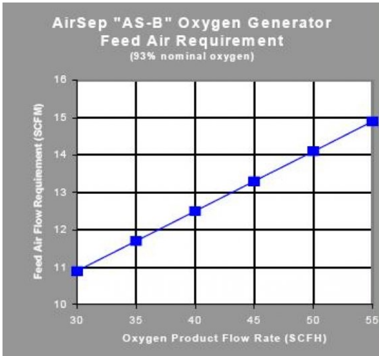
AS-B Performance Chart
